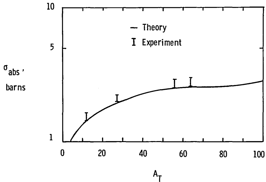
Figure 19. Absorption cross sections, as a function of target mass number, for neon projectiles at 30 MeV/nucleon.
